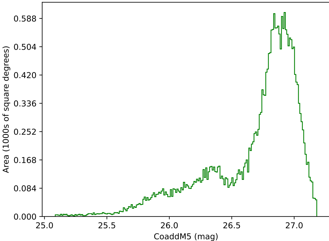
weather_cloudso2v3.4_10yrs All sky g band: CoaddM5
