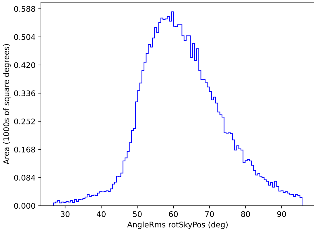
weather_cloudso2v3.4_10yrs All sky u band: AngleRms rotSkyPos
