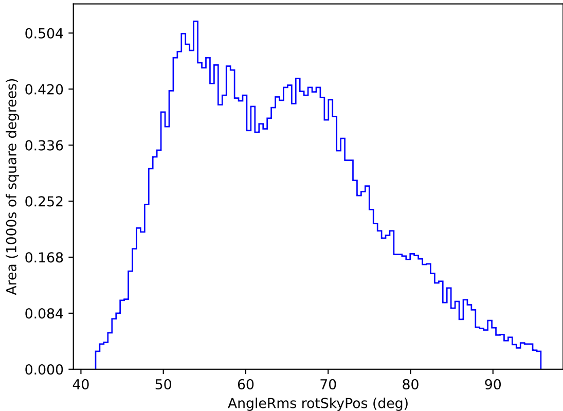
weather_cloudso2v3.4_10yrs All sky r band: AngleRms rotSkyPos
