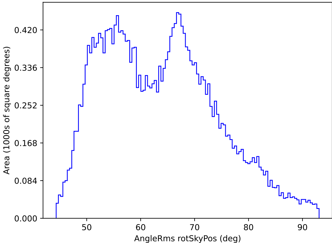
weather_cloudso2v3.4_10yrs All sky all bands: AngleRms rotSkyPos
