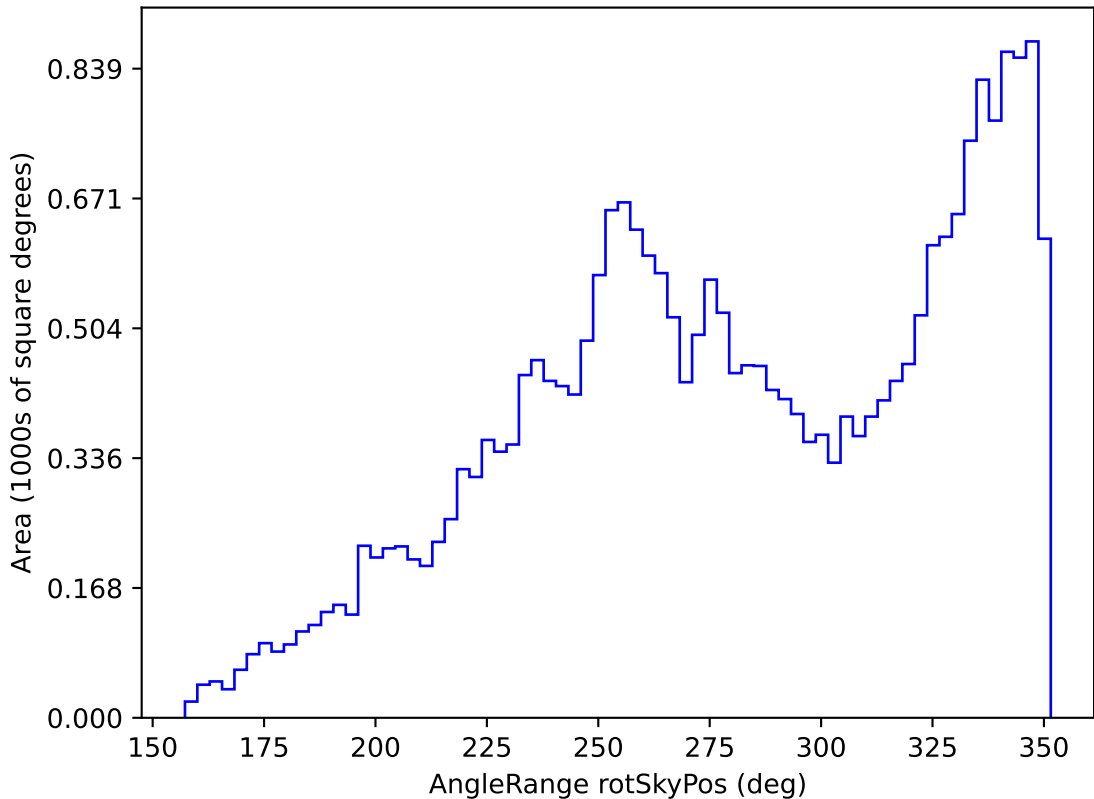
weather_cloudso2v3.4_10yrs All sky all bands: AngleRange rotSkyPos
