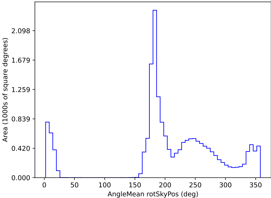
weather_cloudso2v3.4_10yrs WFD all bands: AngleMean rotSkyPos
