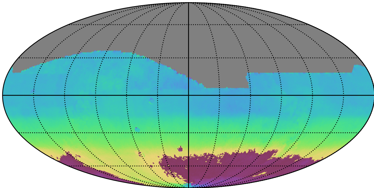
weather_cloudso2v3.4_10yrs All sky all bands: AngleMean rotSkyPos
