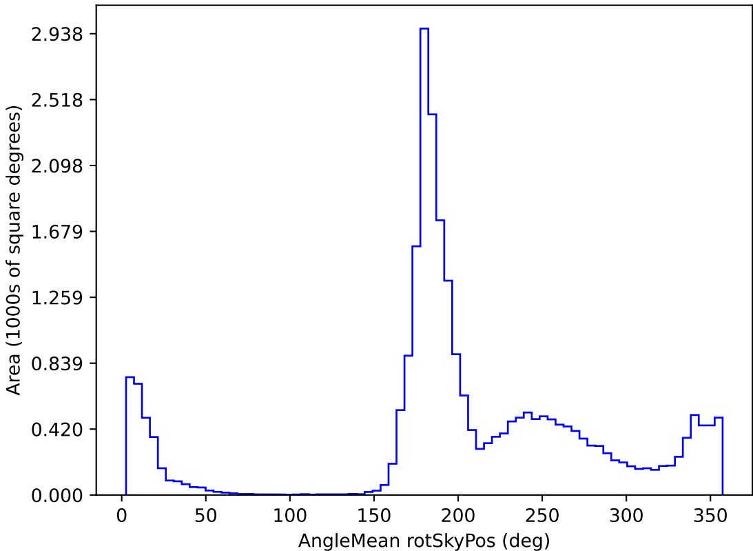
weather_cloudso2v3.4_10yrs All sky all bands: AngleMean rotSkyPos
