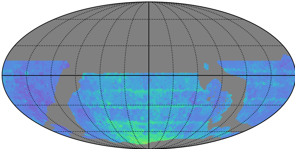
weather_cloudso2v3.4_10yrs WFD y band: 80thPercentile Season Length
