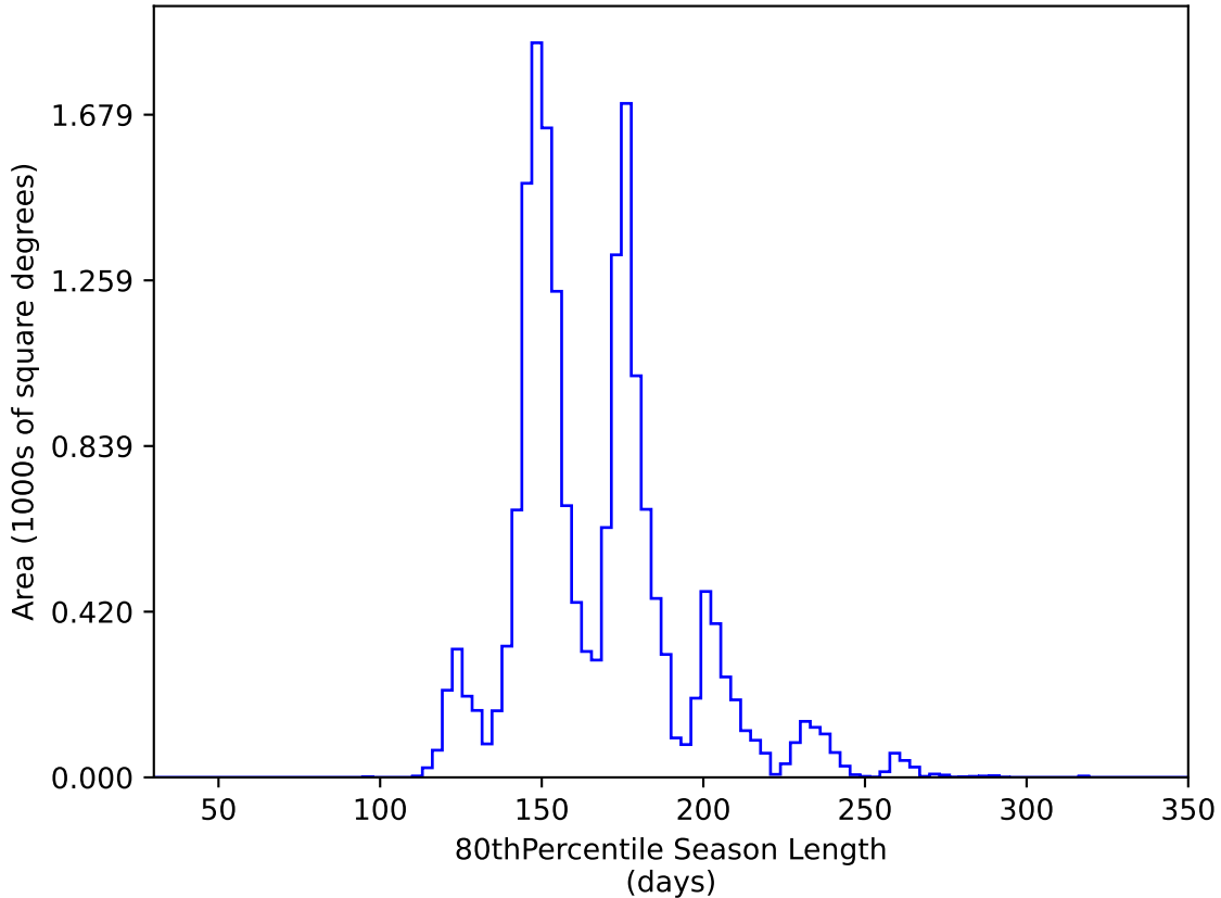
weather_cloudso2v3.4_10yrs WFD y band: 80thPercentile Season Length
