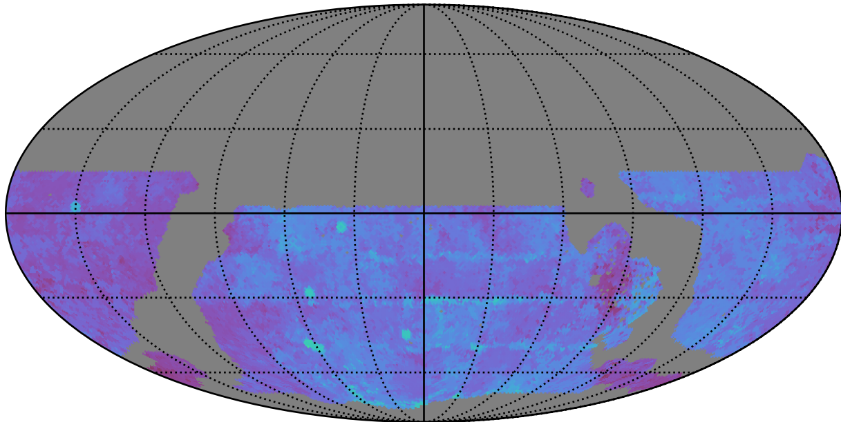
weather_cloudso2v3.4_10yrs WFD u band: 80thPercentile Season Length
