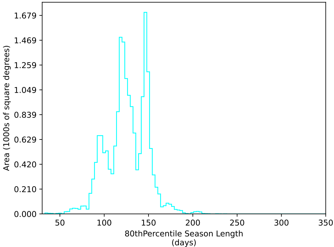
weather_cloudso2v3.4_10yrs WFD u band: 80thPercentile Season Length
