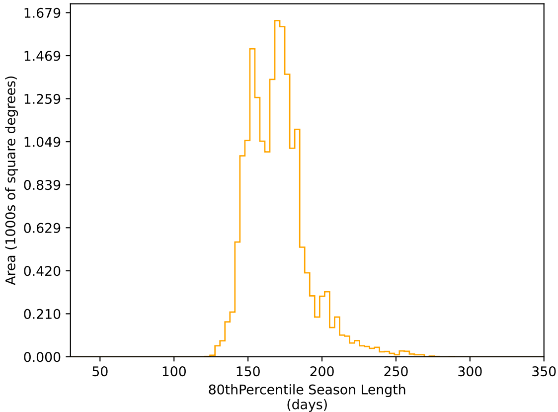
weather_cloudso2v3.4_10yrs WFD r band: 80thPercentile Season Length
