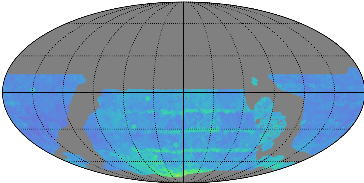
weather_cloudso2v3.4_10yrs WFD i band: 80thPercentile Season Length
