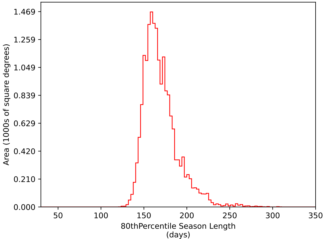
weather_cloudso2v3.4_10yrs WFD i band: 80thPercentile Season Length
