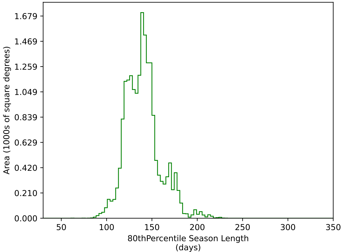
weather_cloudso2v3.4_10yrs WFD g band: 80thPercentile Season Length
