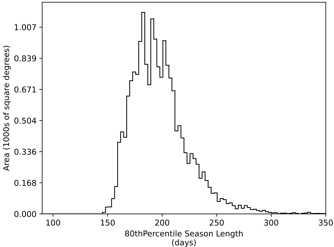
weather_cloudso2v3.4_10yrs WFD all bands: 80thPercentile Season Length
