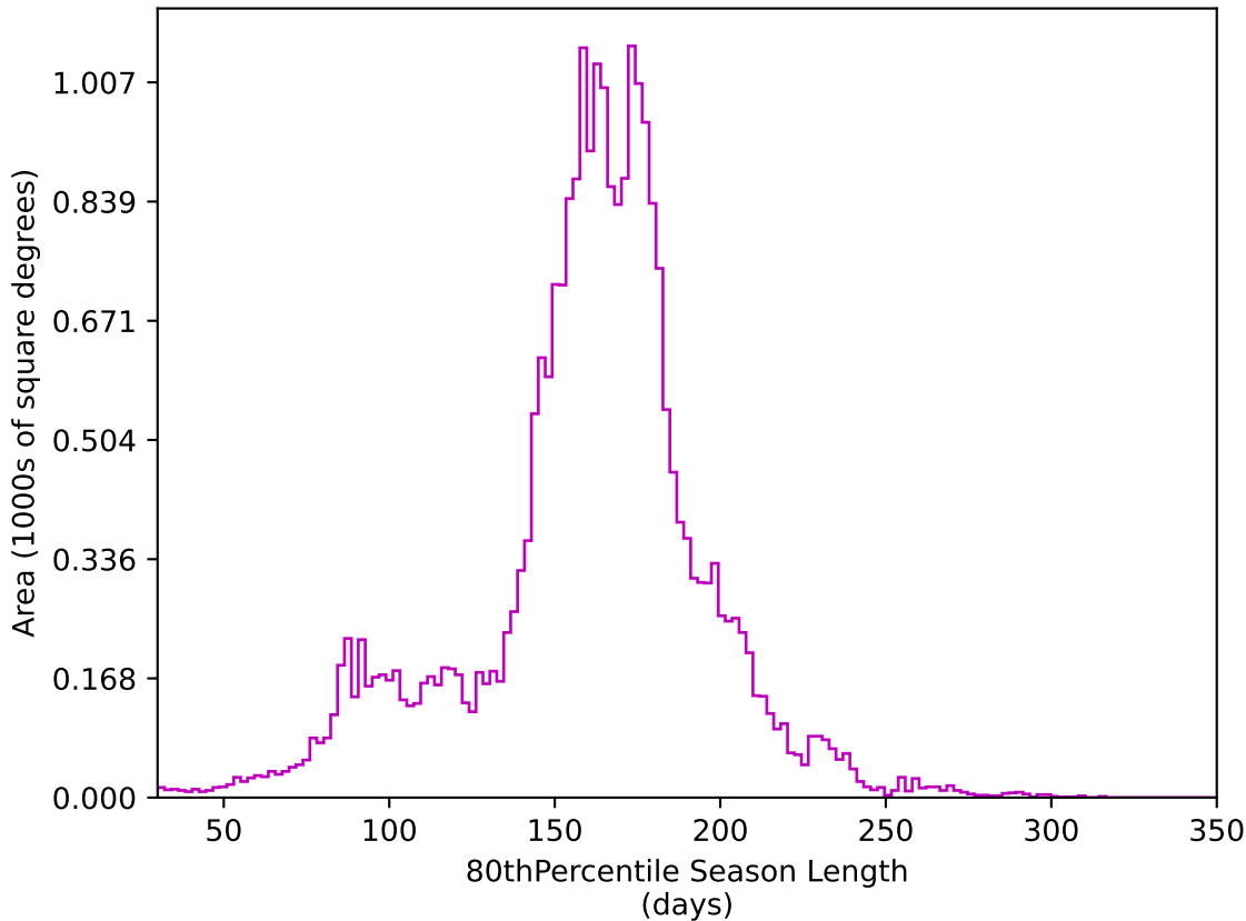
weather_cloudso2v3.4_10yrs All sky z band: 80thPercentile Season Length
