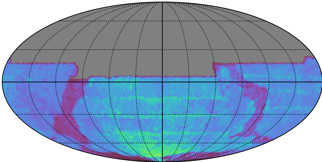
weather_cloudso2v3.4_10yrs All sky y band: 80thPercentile Season Length
