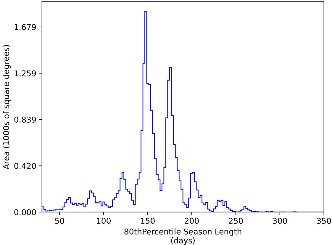
weather_cloudso2v3.4_10yrs All sky y band: 80thPercentile Season Length
