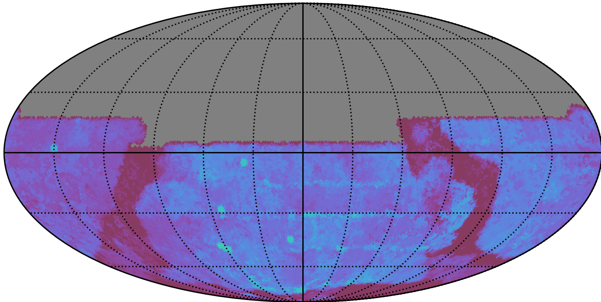
weather_cloudso2v3.4_10yrs All sky u band: 80thPercentile Season Length
