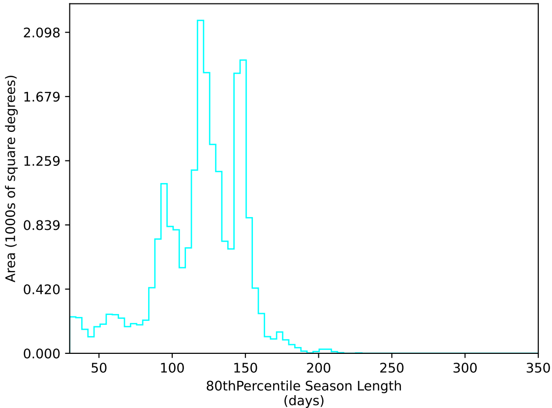
weather_cloudso2v3.4_10yrs All sky u band: 80thPercentile Season Length
