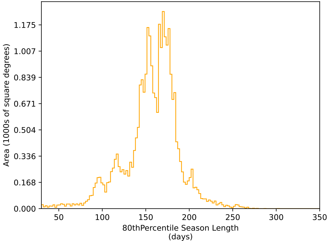
weather_cloudso2v3.4_10yrs All sky r band: 80thPercentile Season Length
