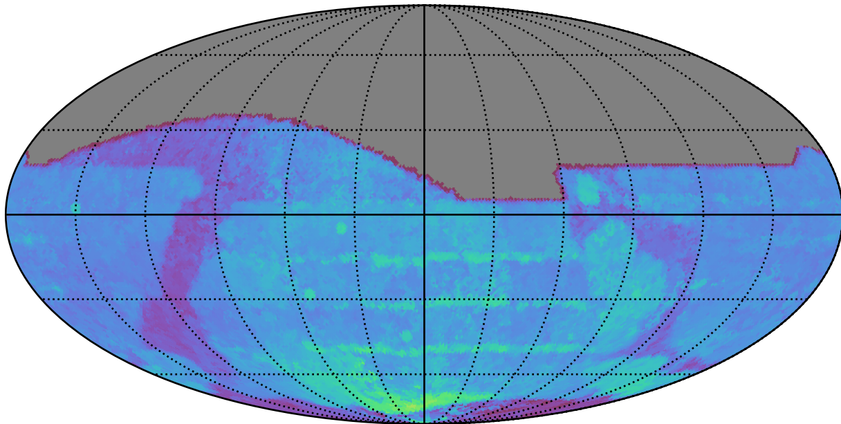
weather_cloudso2v3.4_10yrs All sky i band: 80thPercentile Season Length
