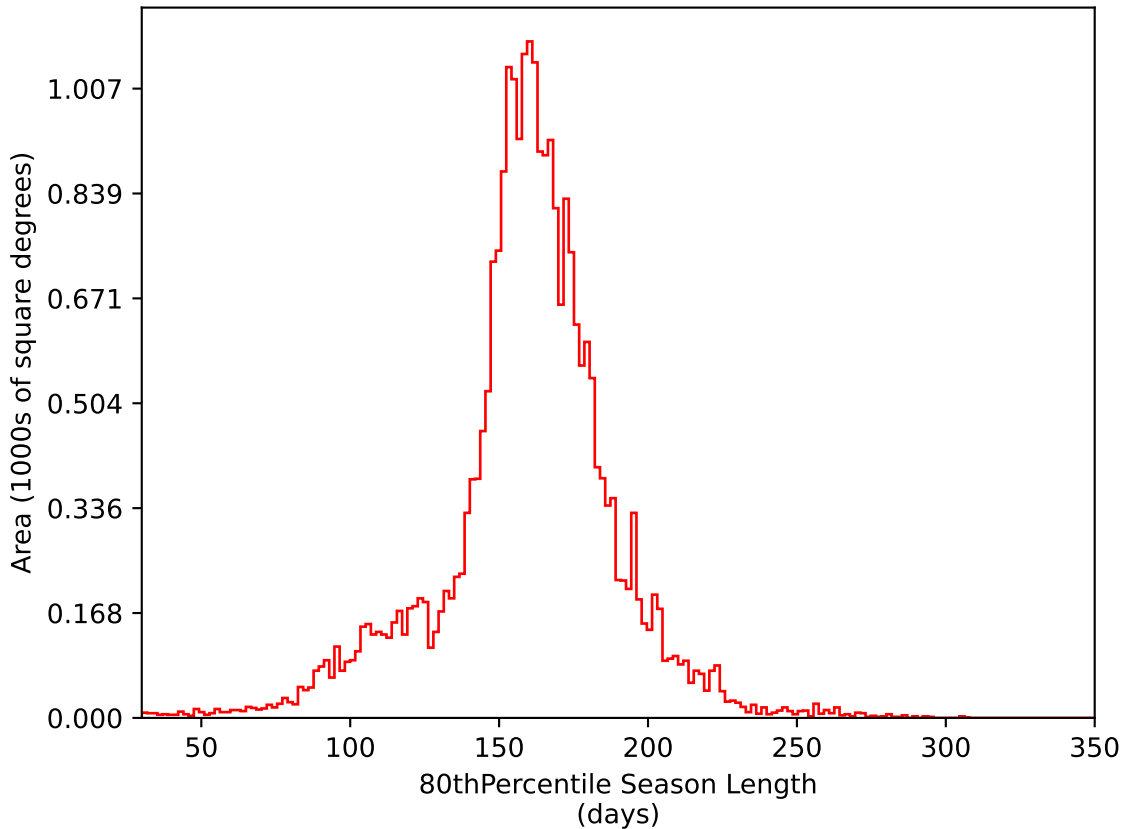
weather_cloudso2v3.4_10yrs All sky i band: 80thPercentile Season Length
