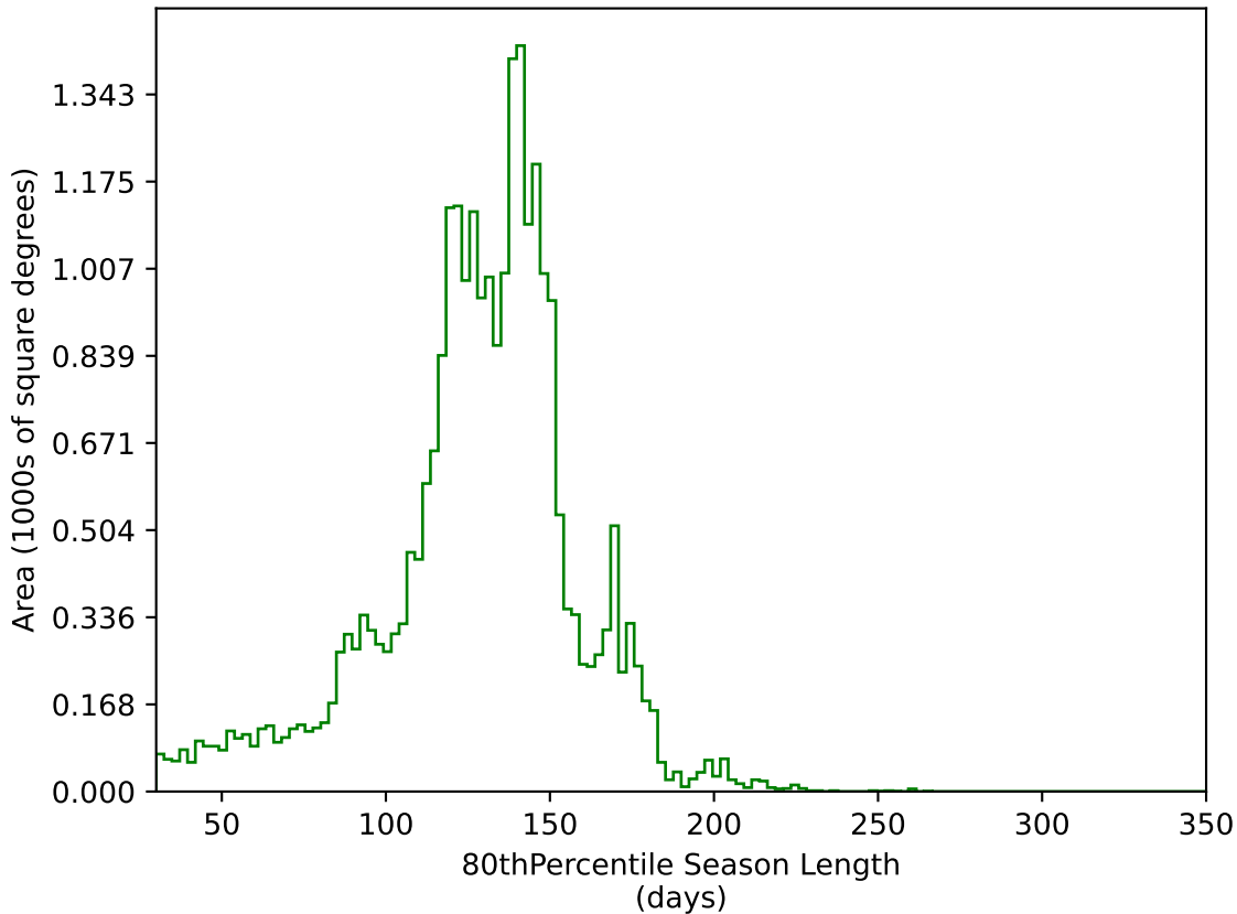
weather_cloudso2v3.4_10yrs All sky g band: 80thPercentile Season Length
