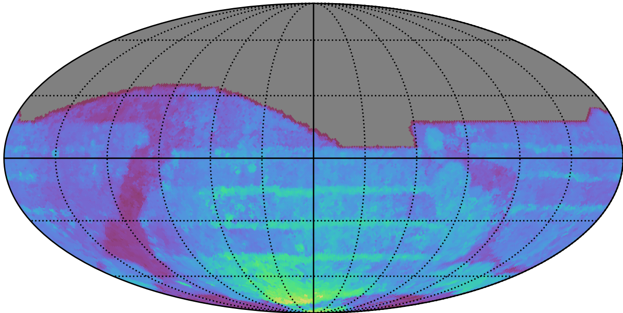
weather_cloudso2v3.4_10yrs All sky all bands: 80thPercentile Season Length
