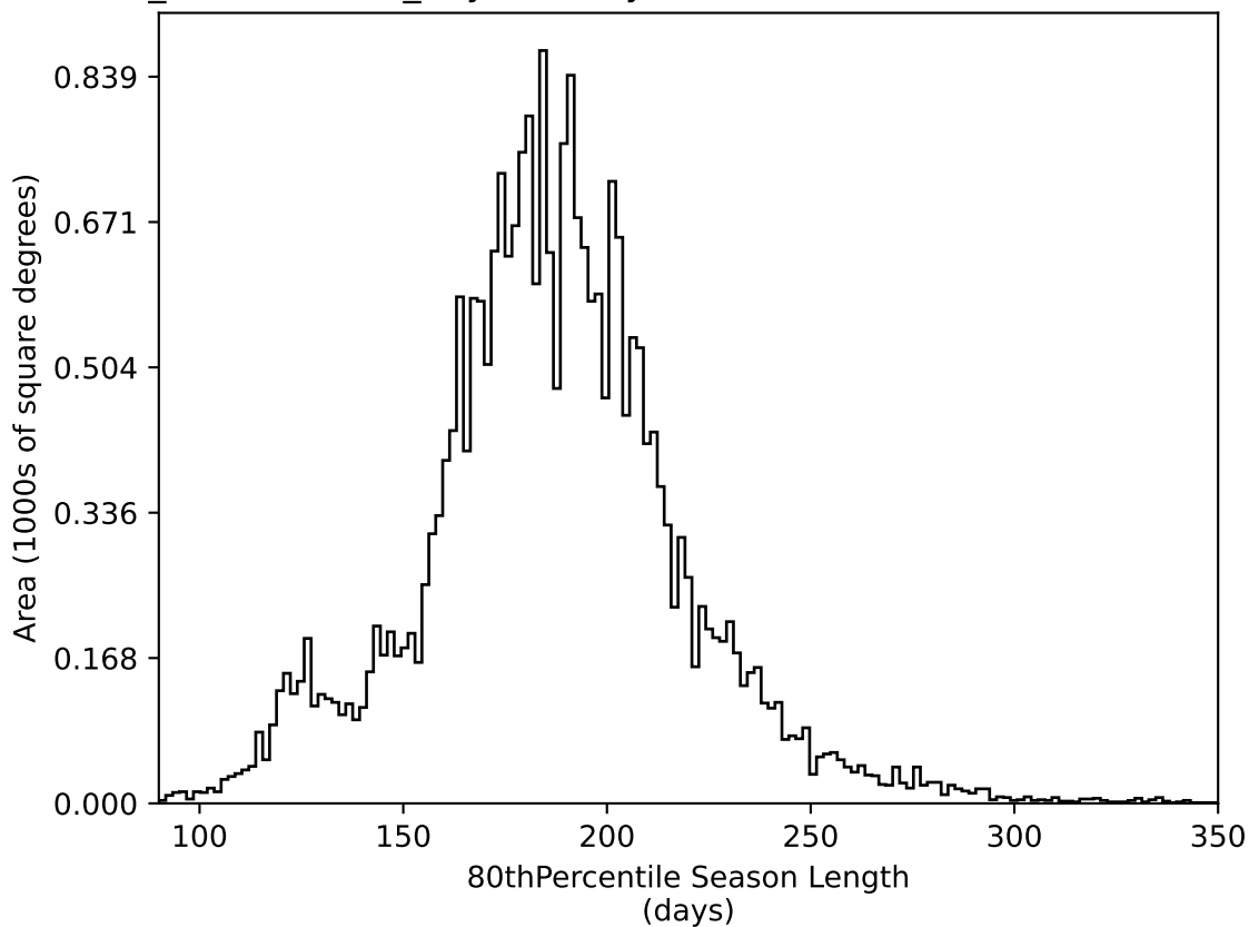
weather_cloudso2v3.4_10yrs All sky all bands: 80thPercentile Season Length
