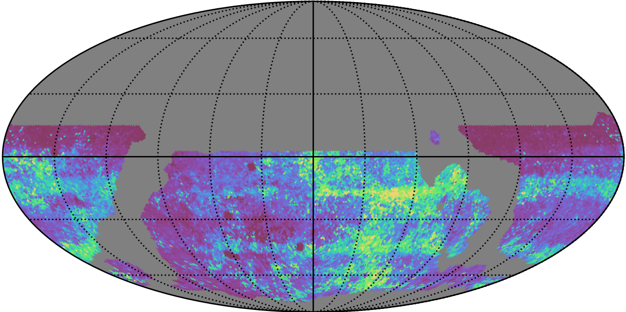
weather_cloudso2v3.4_10yrs WFD zy bands: 75th Percentile Intranight Timespan
