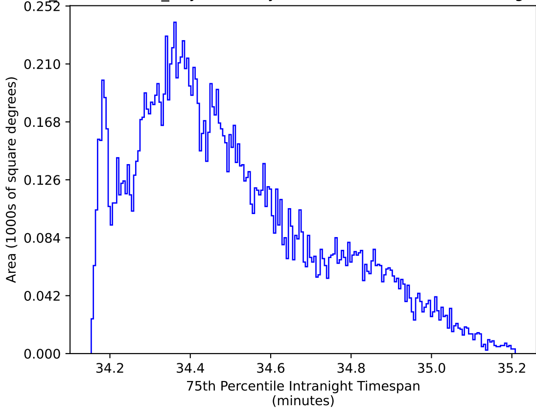
weather_cloudso2v3.4_10yrs WFD zy bands: 75th Percentile Intranight Timespan
