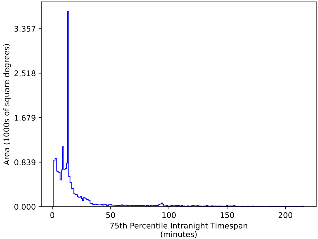
weather_cloudso2v3.4_10yrs WFD z band: 75th Percentile Intranight Timespan
