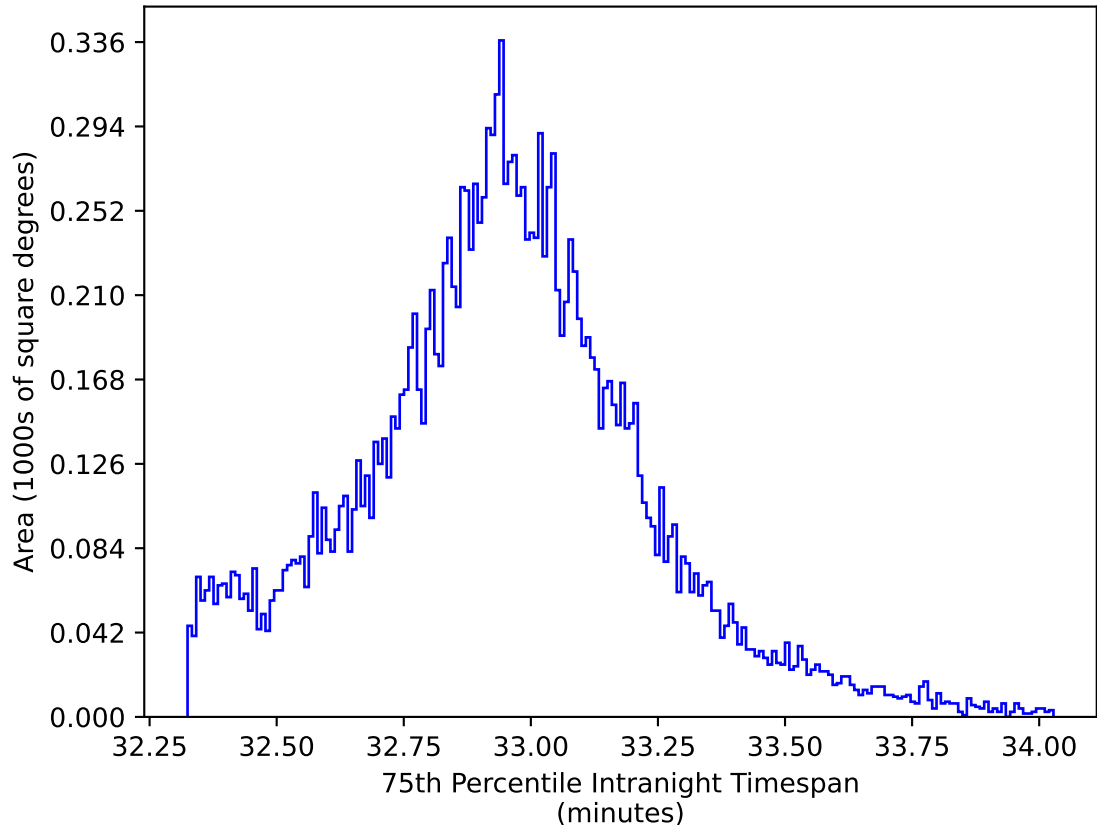
weather_cloudso2v3.4_10yrs WFD y band: 75th Percentile Intranight Timespan
