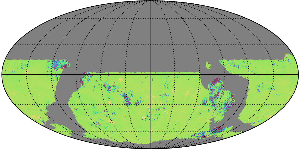
weather_cloudso2v3.4_10yrs WFD ug bands: 75th Percentile Intranight Timespan
