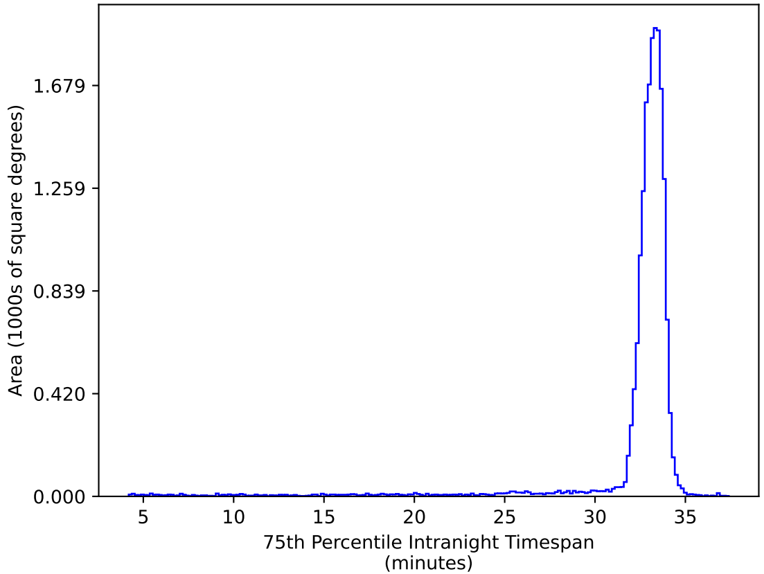
weather_cloudso2v3.4_10yrs WFD ug bands: 75th Percentile Intranight Timespan
