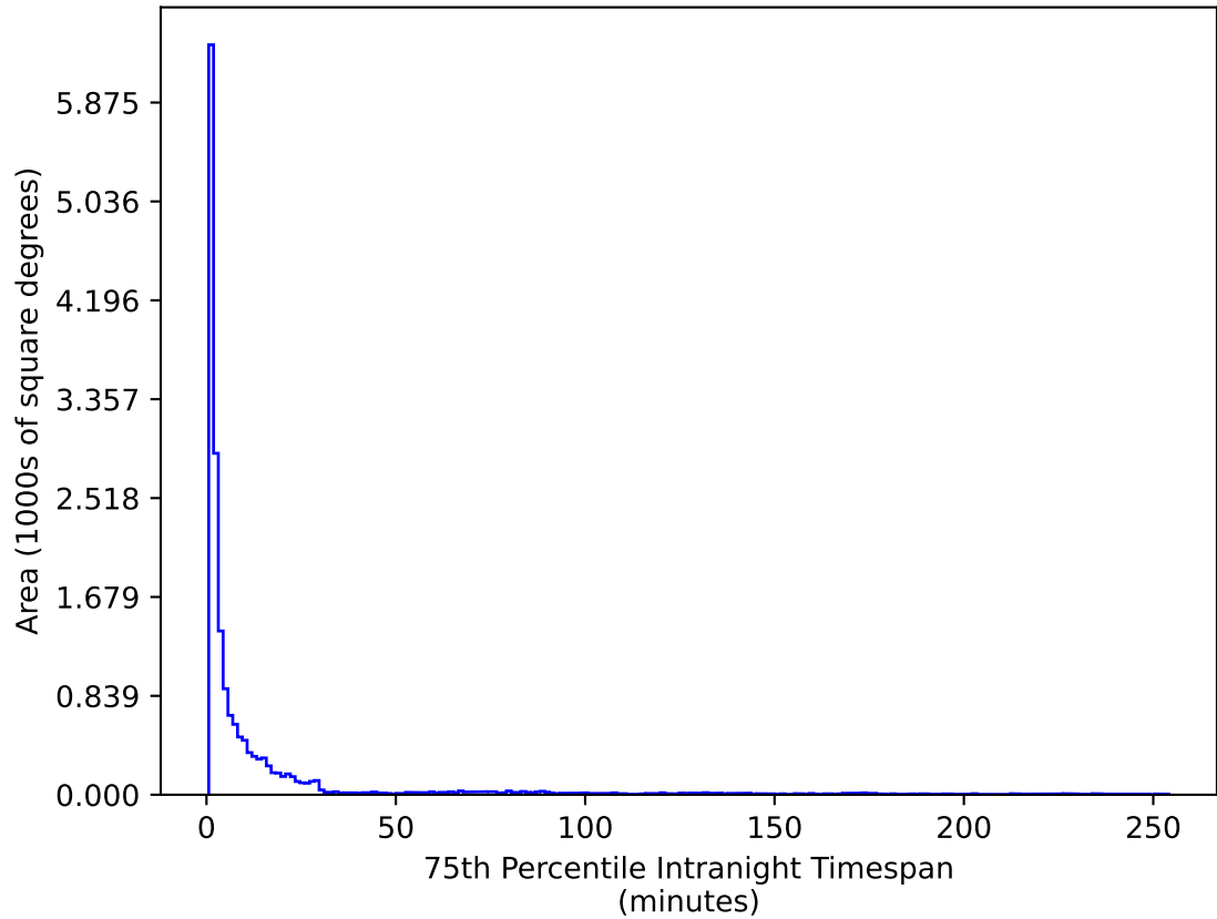
weather_cloudso2v3.4_10yrs WFD u band: 75th Percentile Intranight Timespan
