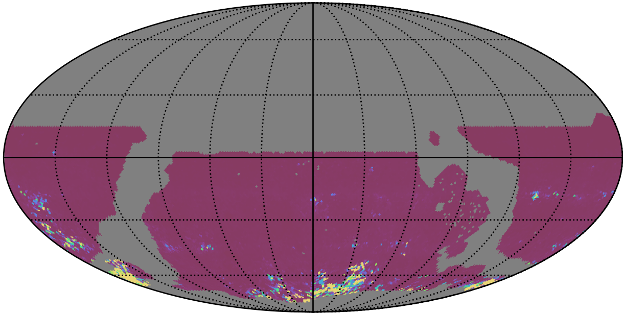
weather_cloudso2v3.4_10yrs WFD ri bands: 75th Percentile Intranight Timespan
