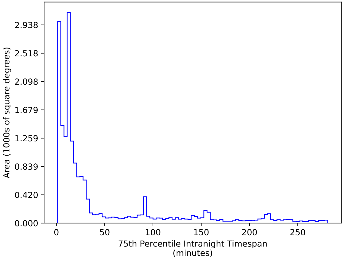
weather_cloudso2v3.4_10yrs WFD r band: 75th Percentile Intranight Timespan
