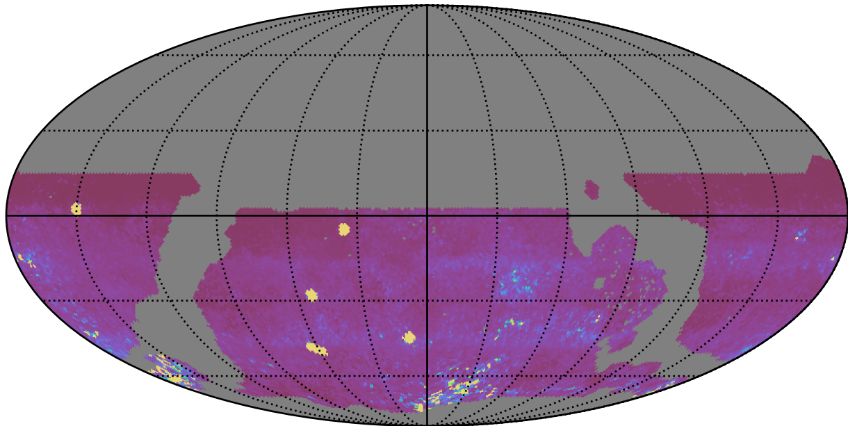
weather_cloudso2v3.4_10yrs WFD iz bands: 75th Percentile Intranight Timespan
