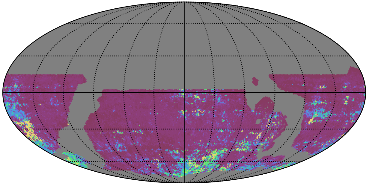
weather_cloudso2v3.4_10yrs WFD i band: 75th Percentile Intranight Timespan
