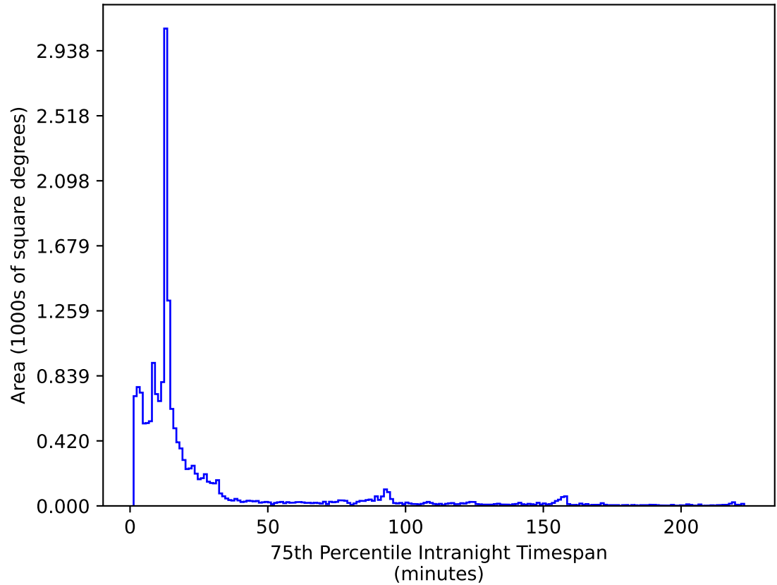
weather_cloudso2v3.4_10yrs WFD i band: 75th Percentile Intranight Timespan
