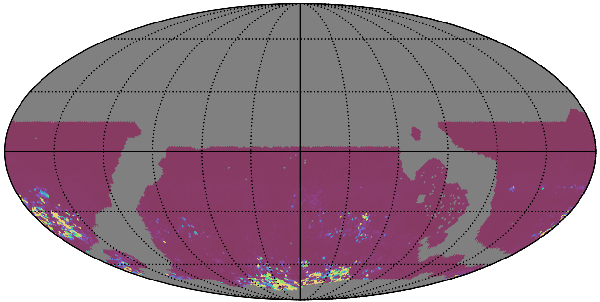
weather_cloudso2v3.4_10yrs WFD gr bands: 75th Percentile Intranight Timespan
