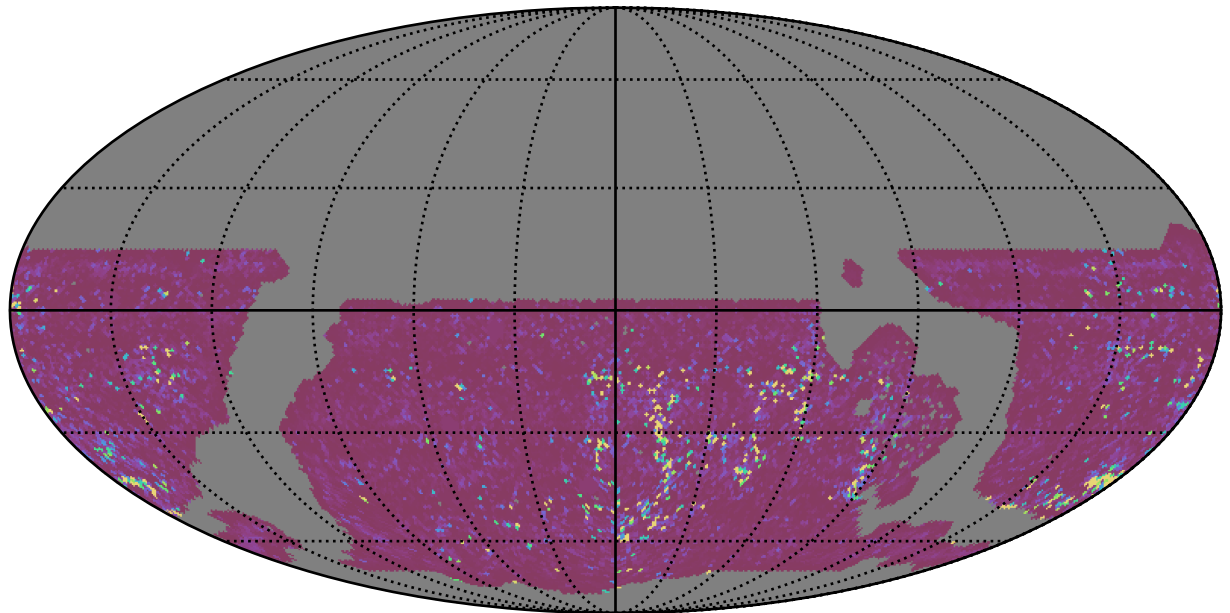
weather_cloudso2v3.4_10yrs WFD g band: 75th Percentile Intranight Timespan
