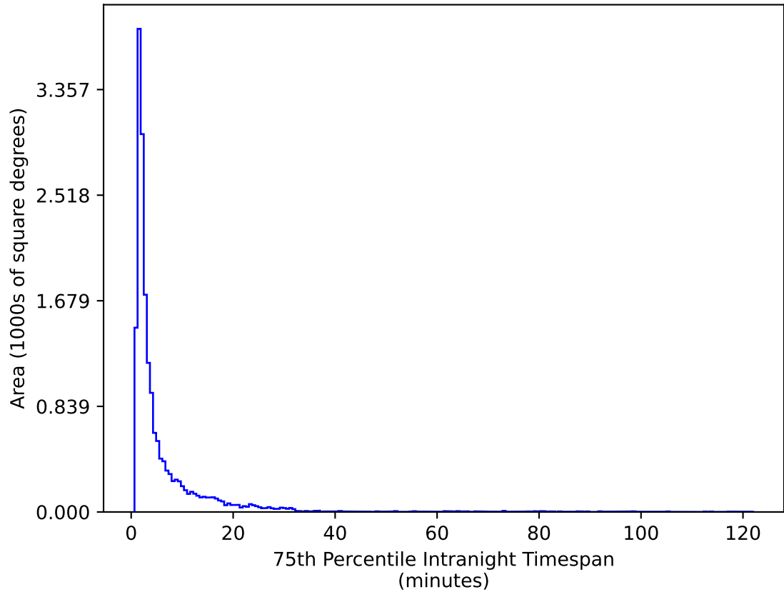
weather_cloudso2v3.4_10yrs WFD g band: 75th Percentile Intranight Timespan
