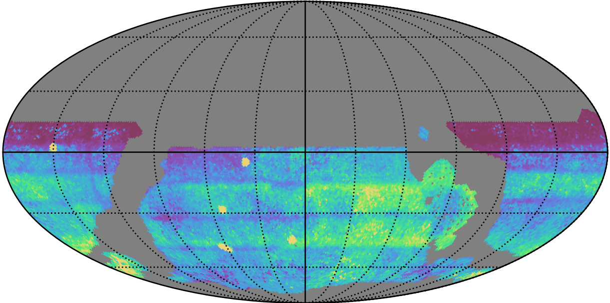
weather_cloudso2v3.4_10yrs WFD all bands: 75th Percentile Intranight Timespan
