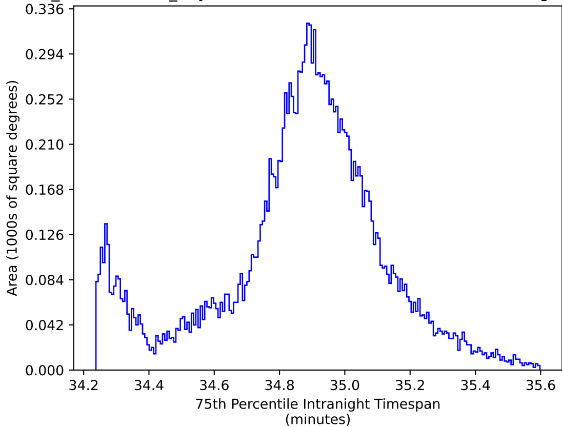
weather_cloudso2v3.4_10yrs WFD all bands: 75th Percentile Intranight Timespan
