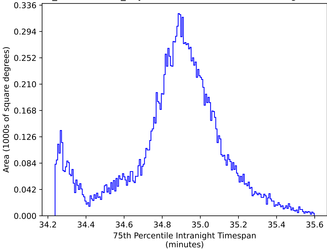
weather_cloudso2v3.4_10yrs WFD: 75th Percentile Intranight Timespan
