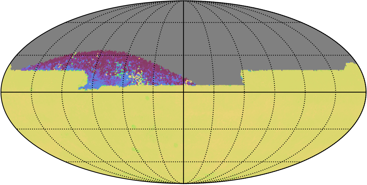
weather_cloudso2v3.4_10yrs All sky zy bands: 75th Percentile Intranight Timespan
