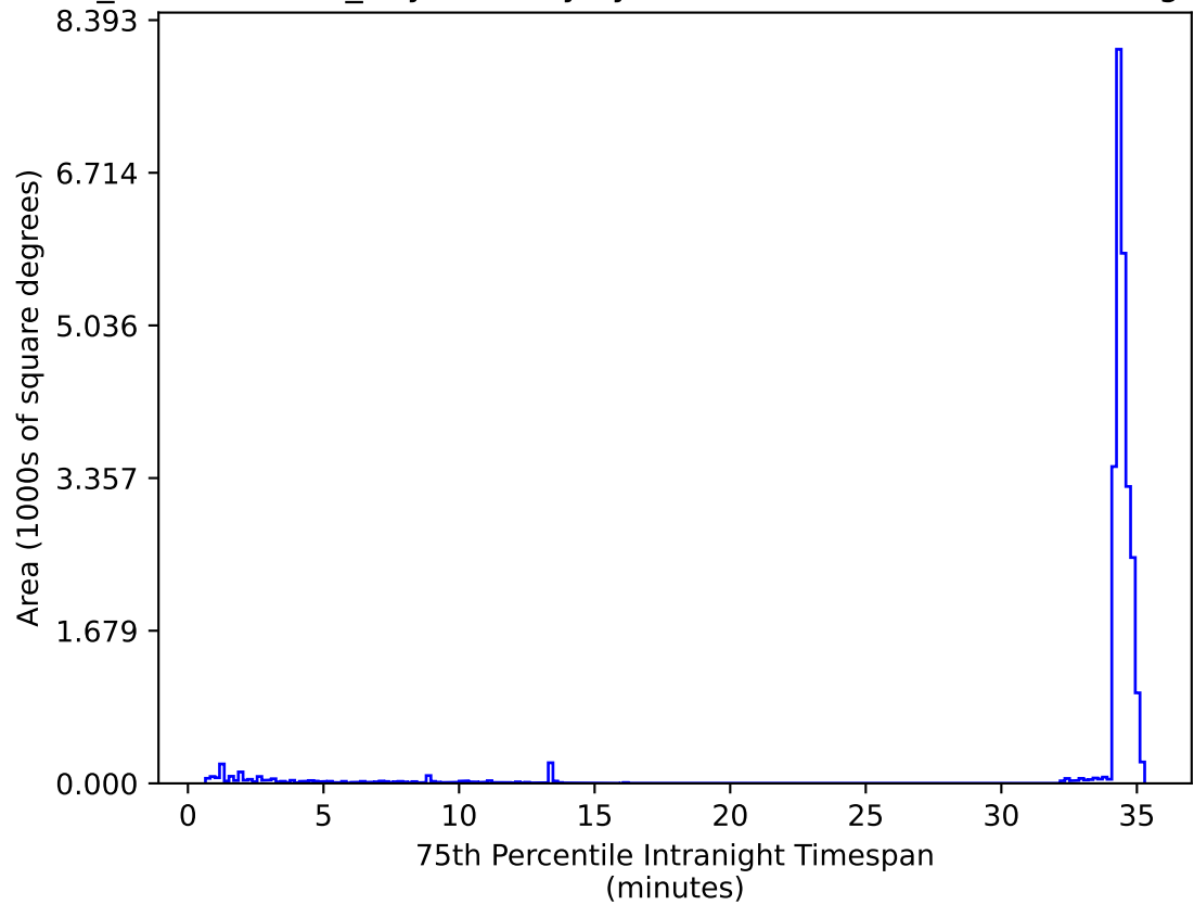
weather_cloudso2v3.4_10yrs All sky zy bands: 75th Percentile Intranight Timespan
