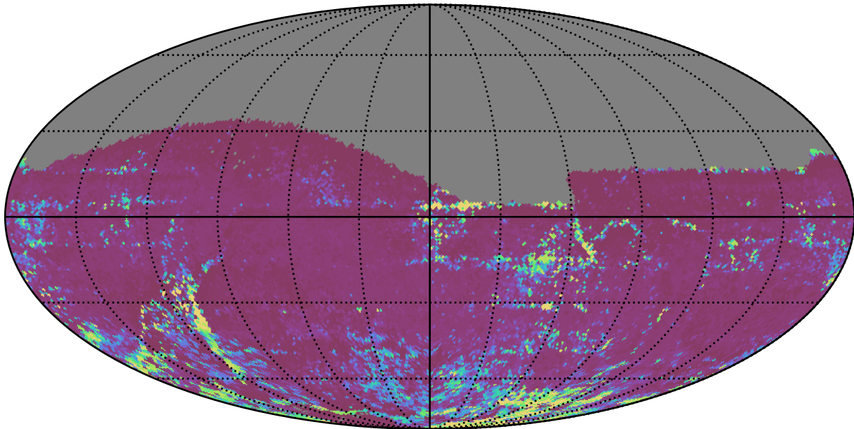
weather_cloudso2v3.4_10yrs All sky z band: 75th Percentile Intranight Timespan
