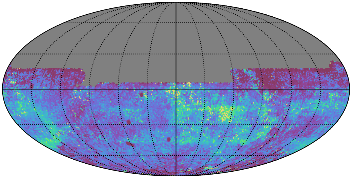
weather_cloudso2v3.4_10yrs All sky y band: 75th Percentile Intranight Timespan
